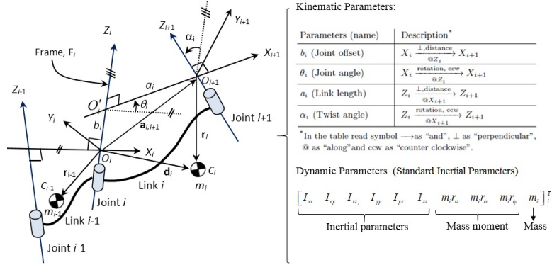
Figure 1: Coordinate frames for spatial two link with its kinematic and dynamic description
