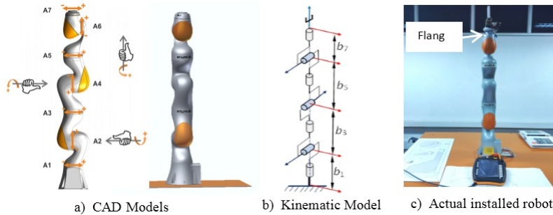
Figure 2: CAD model as in [11] and Autodesk-Inventor, kinematic model and installed robot KUKAiiwa.
